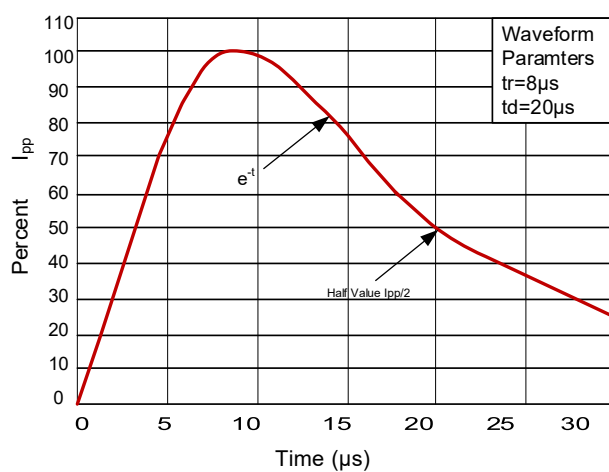
Figure3: Pulse Waveform
